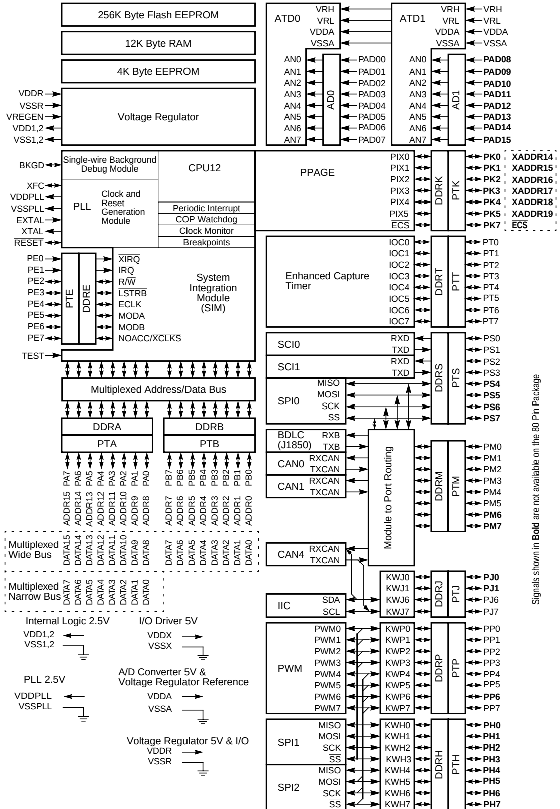
Figure 1-1 MC9S12DT256
